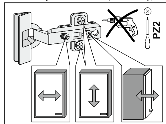
Türverstellungschema (falls erforderlich) Door adjustment scheme (if necessary)
